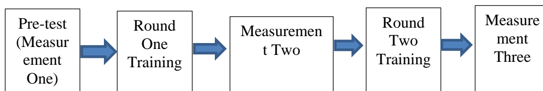
Figure 2: Research Design
